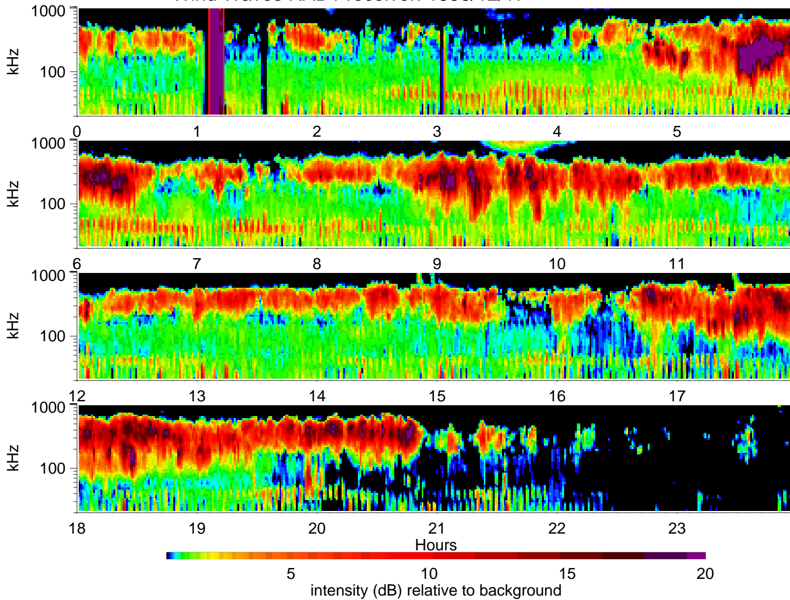
Wind Waves RAD1 receiver: 1996/12/17
