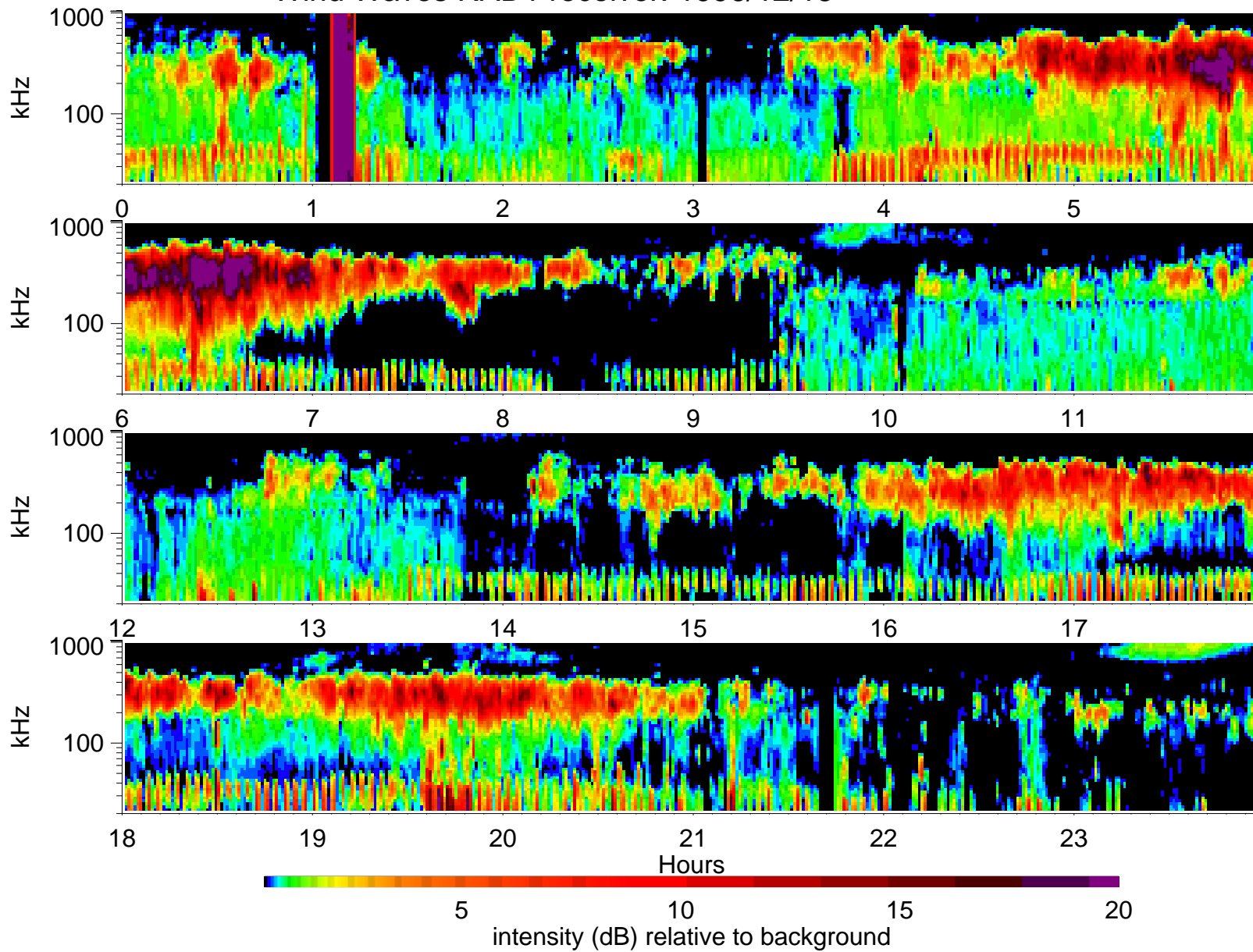
Wind Waves RAD1 receiver: 1996/12/13
