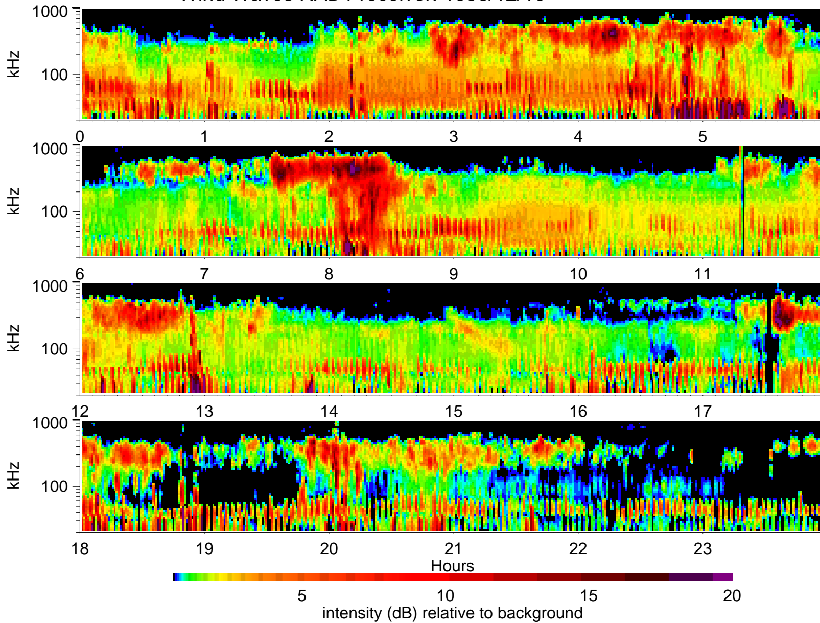
Wind Waves RAD1 receiver: 1996/12/10
