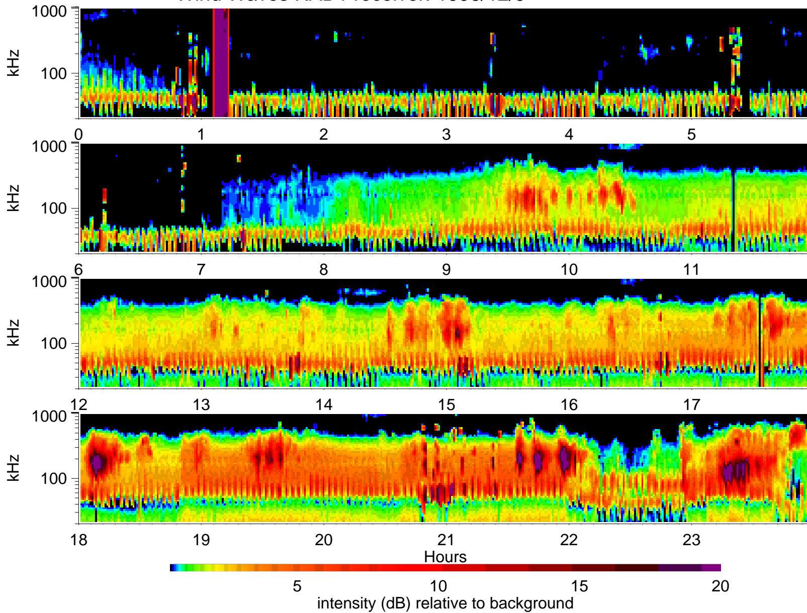
Wind Waves RAD1 receiver: 1996/12/9
