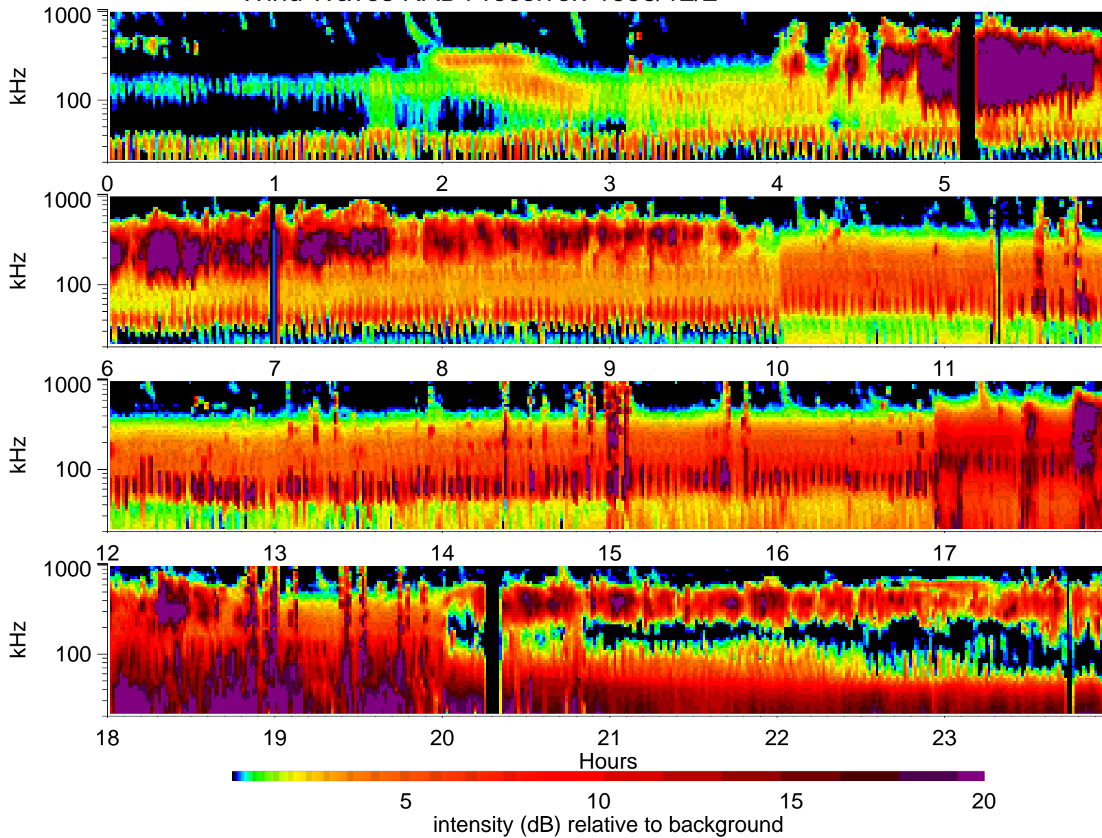
Wind Waves RAD1 receiver: 1996/12/2
