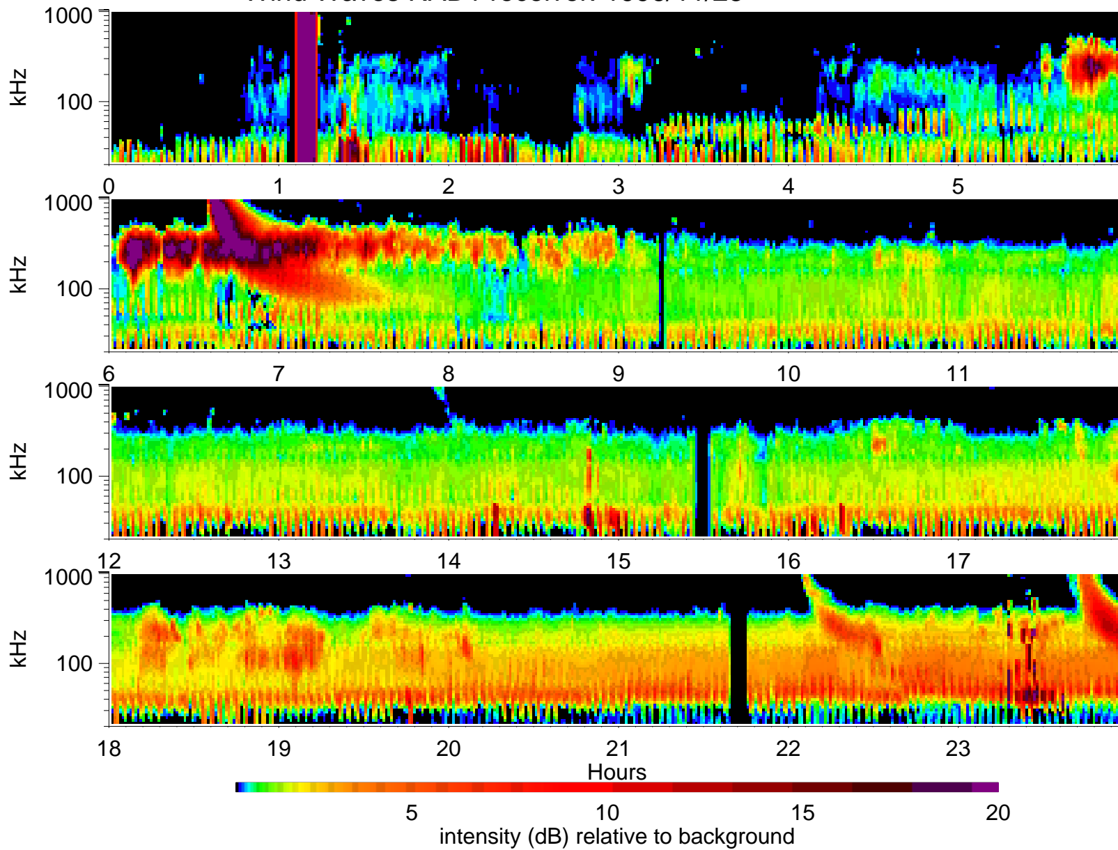
Wind Waves RAD1 receiver: 1996/11/23
