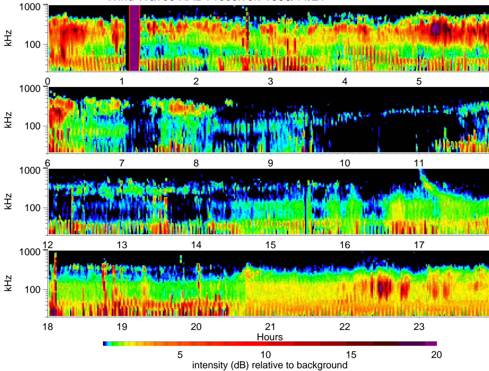
Wind Waves RAD1 receiver: 1996/11/21
