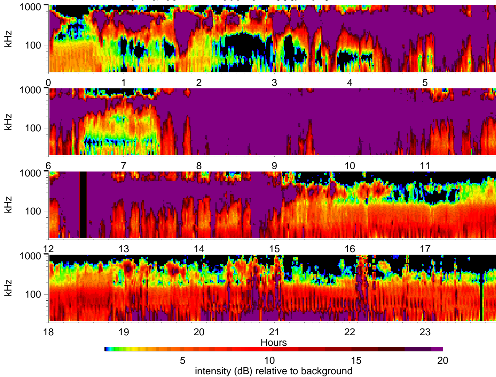
Wind Waves RAD1 receiver: 1996/11/16
