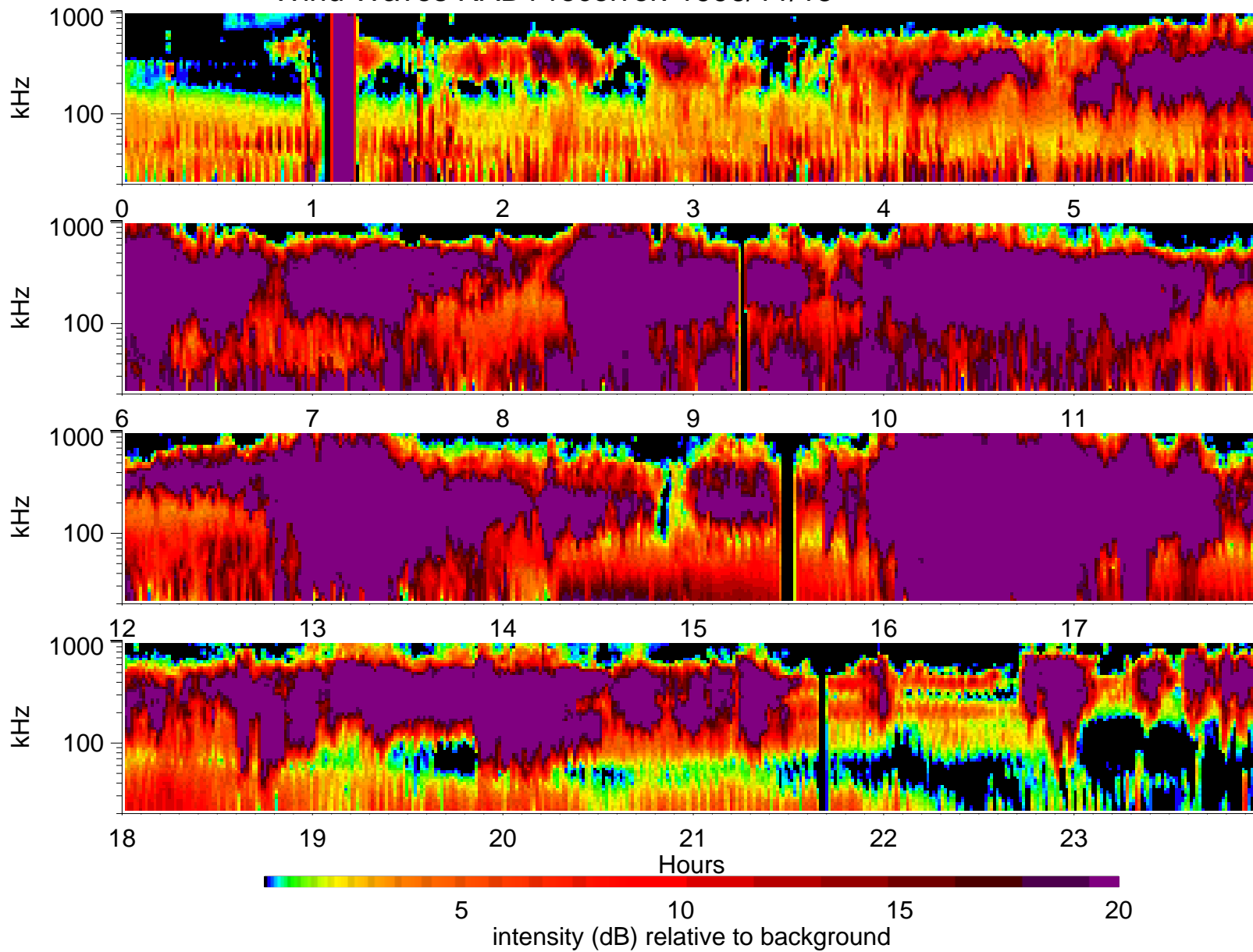
Wind Waves RAD1 receiver: 1996/11/15
