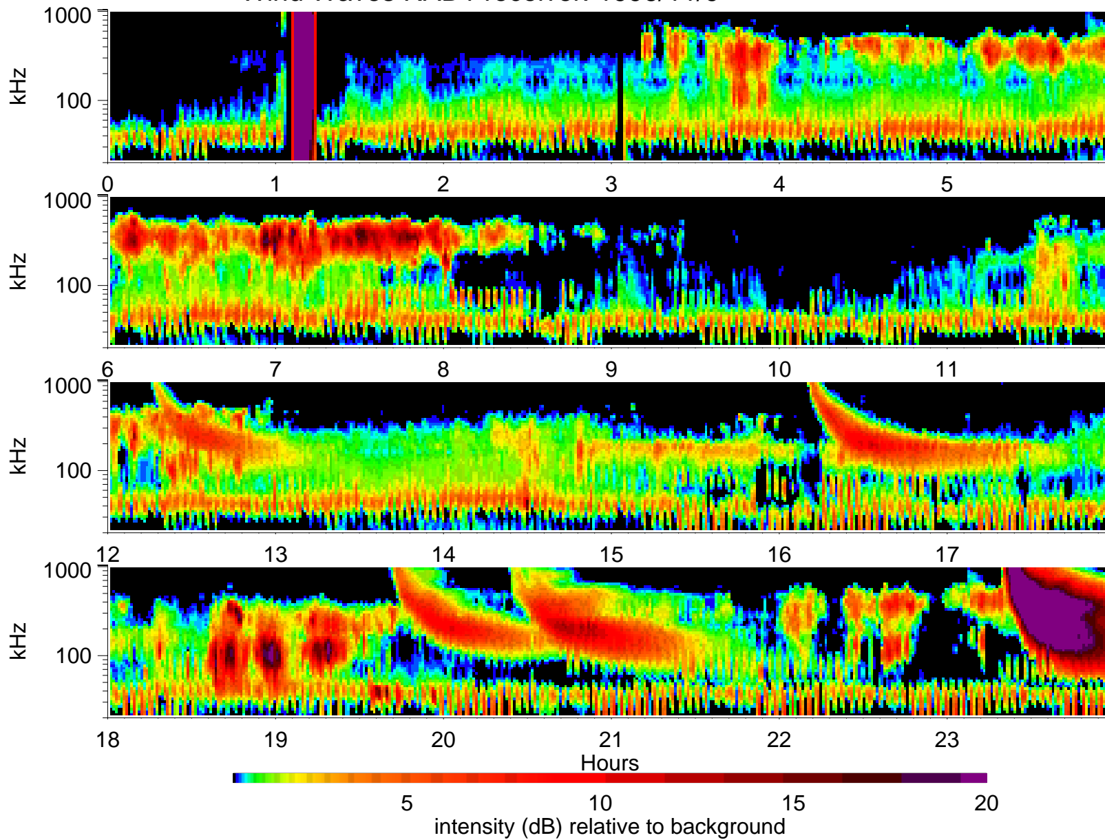
Wind Waves RAD1 receiver: 1996/11/9
