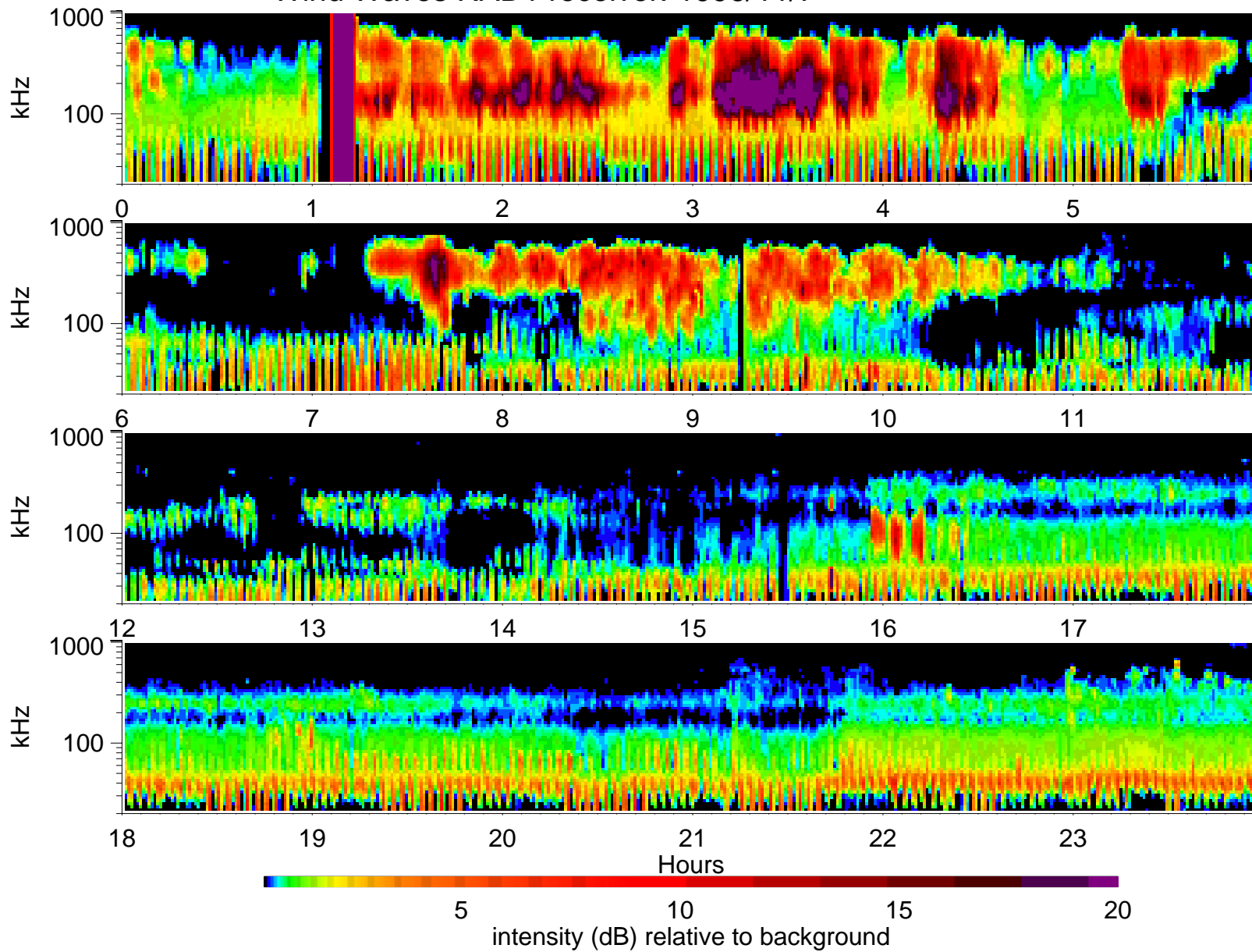
Wind Waves RAD1 receiver: 1996/11/7
