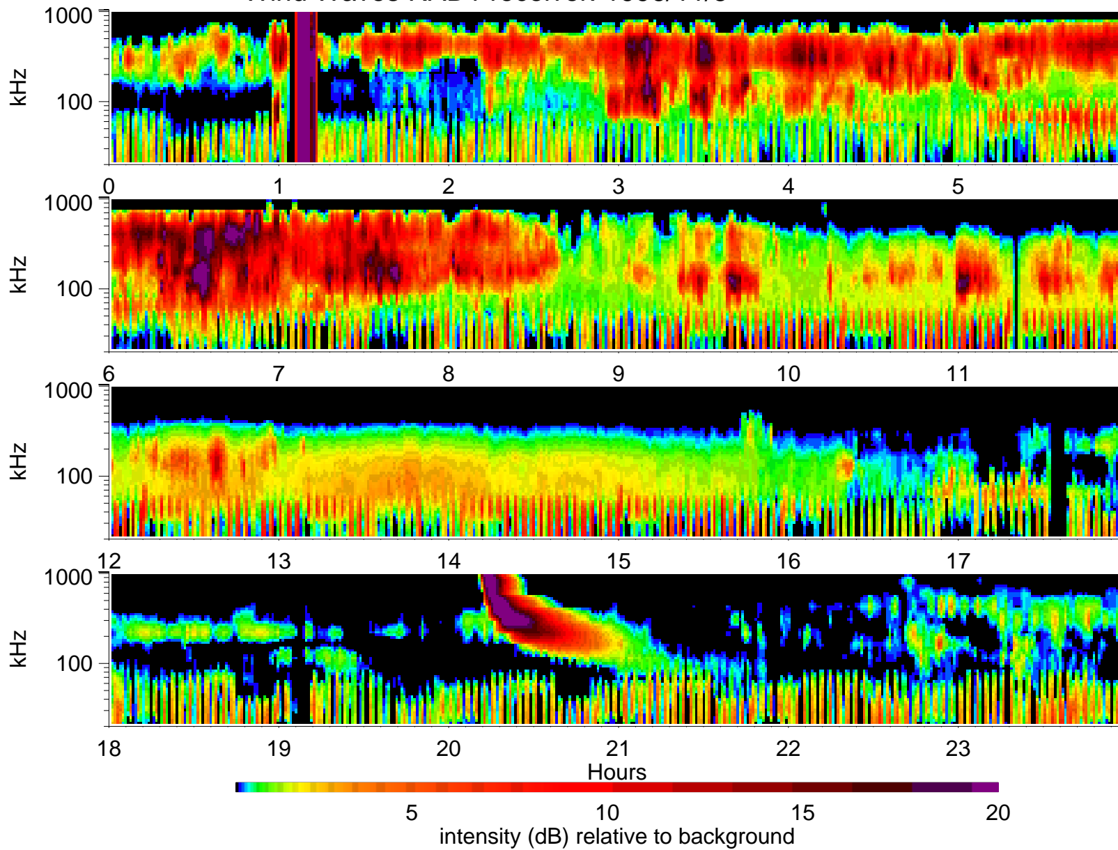
Wind Waves RAD1 receiver: 1996/11/5
