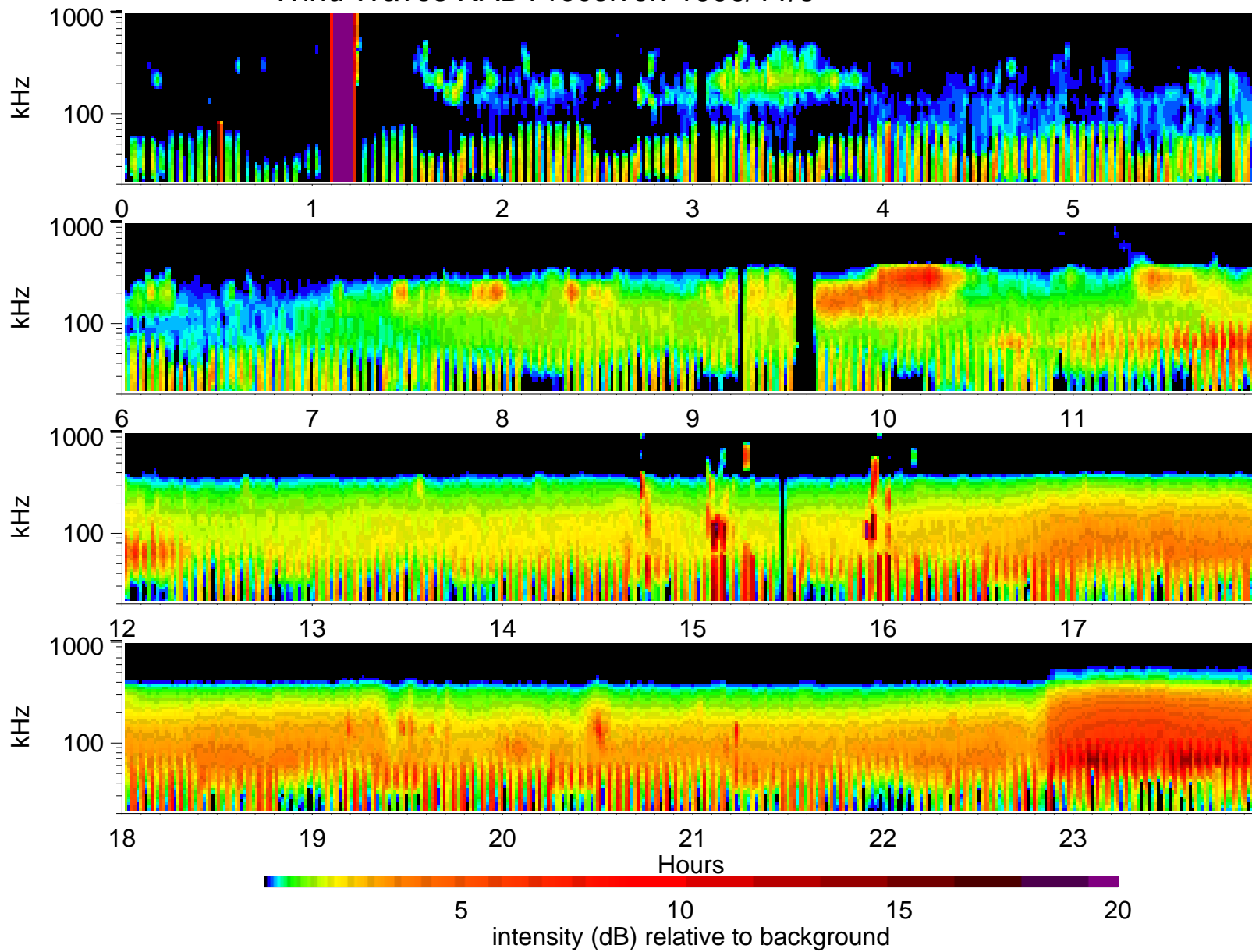
Wind Waves RAD1 receiver: 1996/11/3
