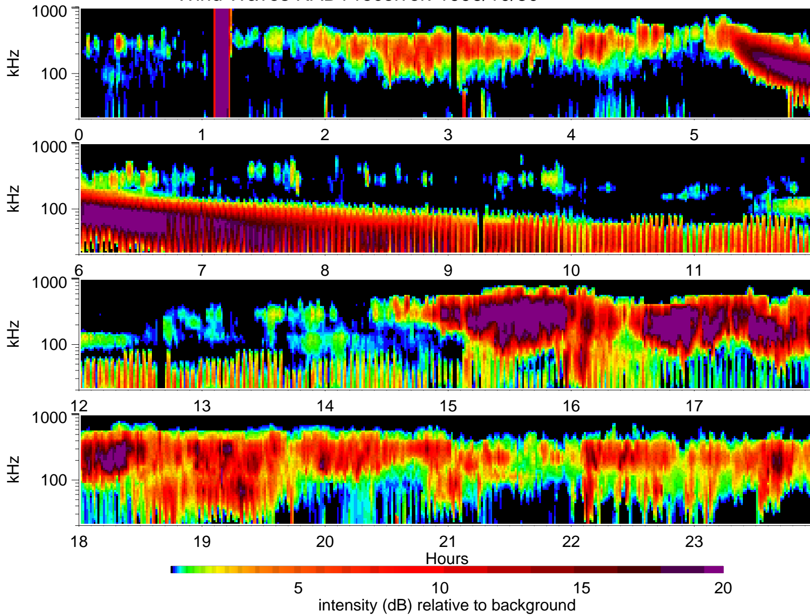
Wind Waves RAD1 receiver: 1996/10/30
