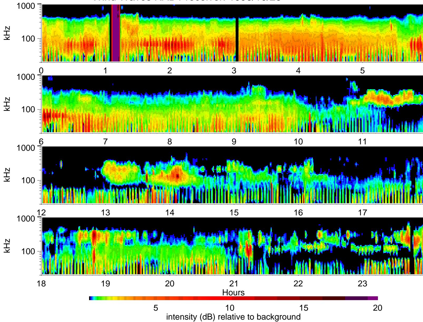
Wind Waves RAD1 receiver: 1996/10/28
