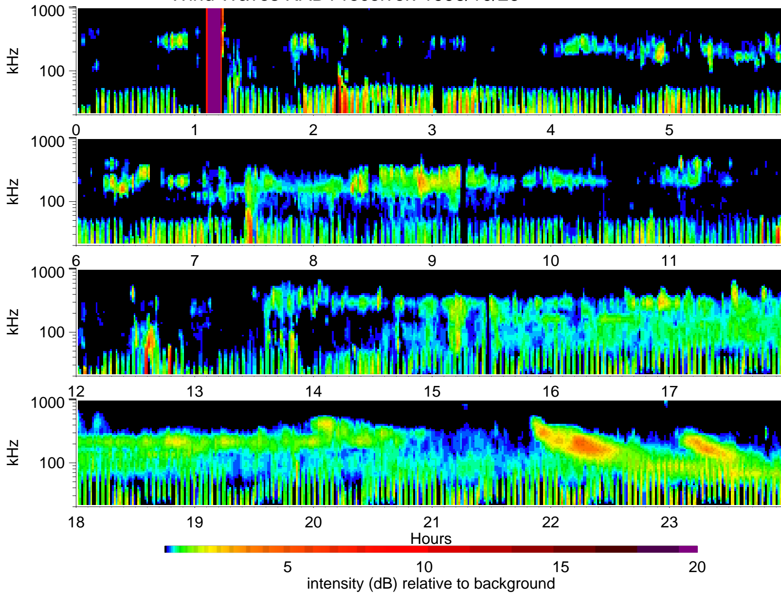
Wind Waves RAD1 receiver: 1996/10/26
