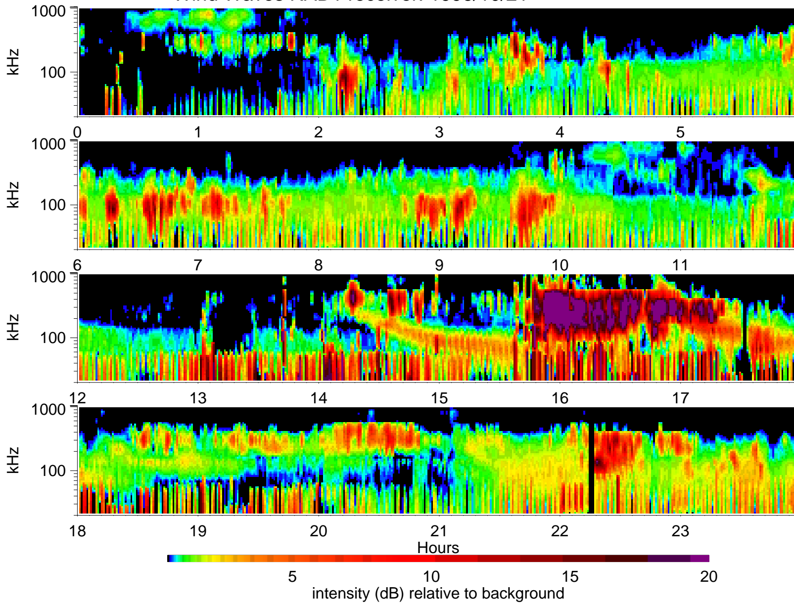
Wind Waves RAD1 receiver: 1996/10/21
