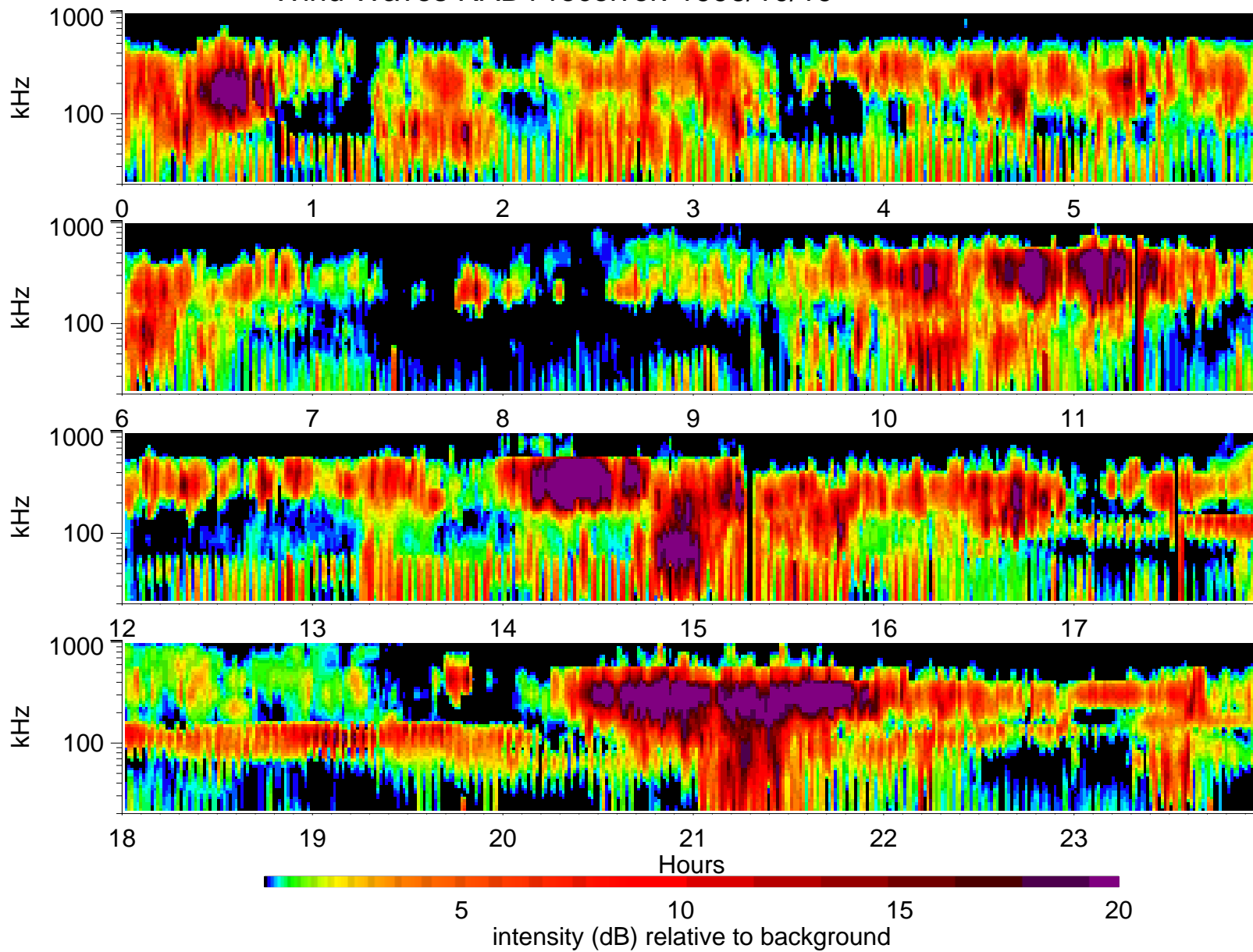
Wind Waves RAD1 receiver: 1996/10/19
