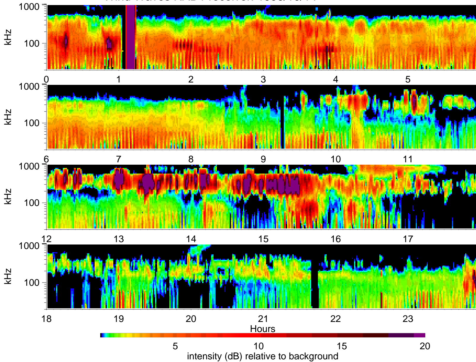
Wind Waves RAD1 receiver: 1996/10/14
