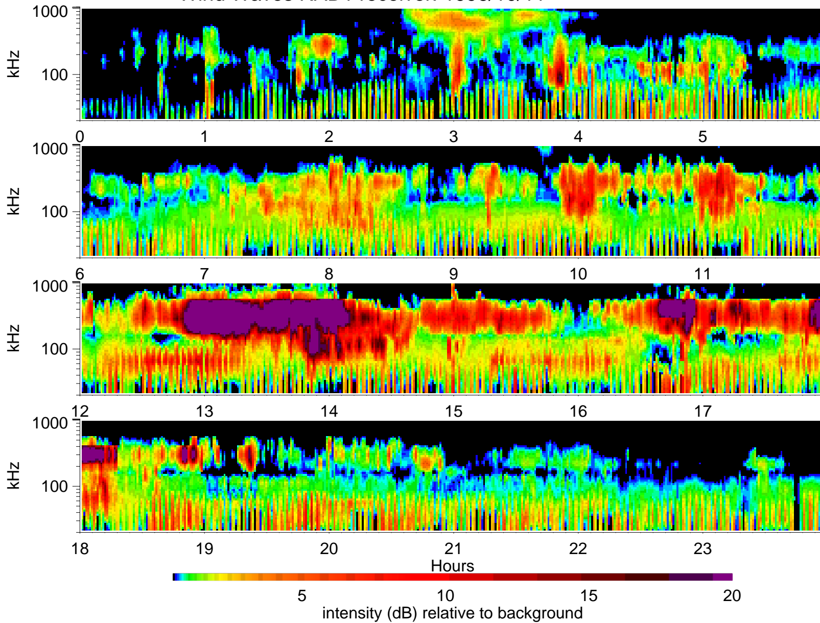
Wind Waves RAD1 receiver: 1996/10/11
