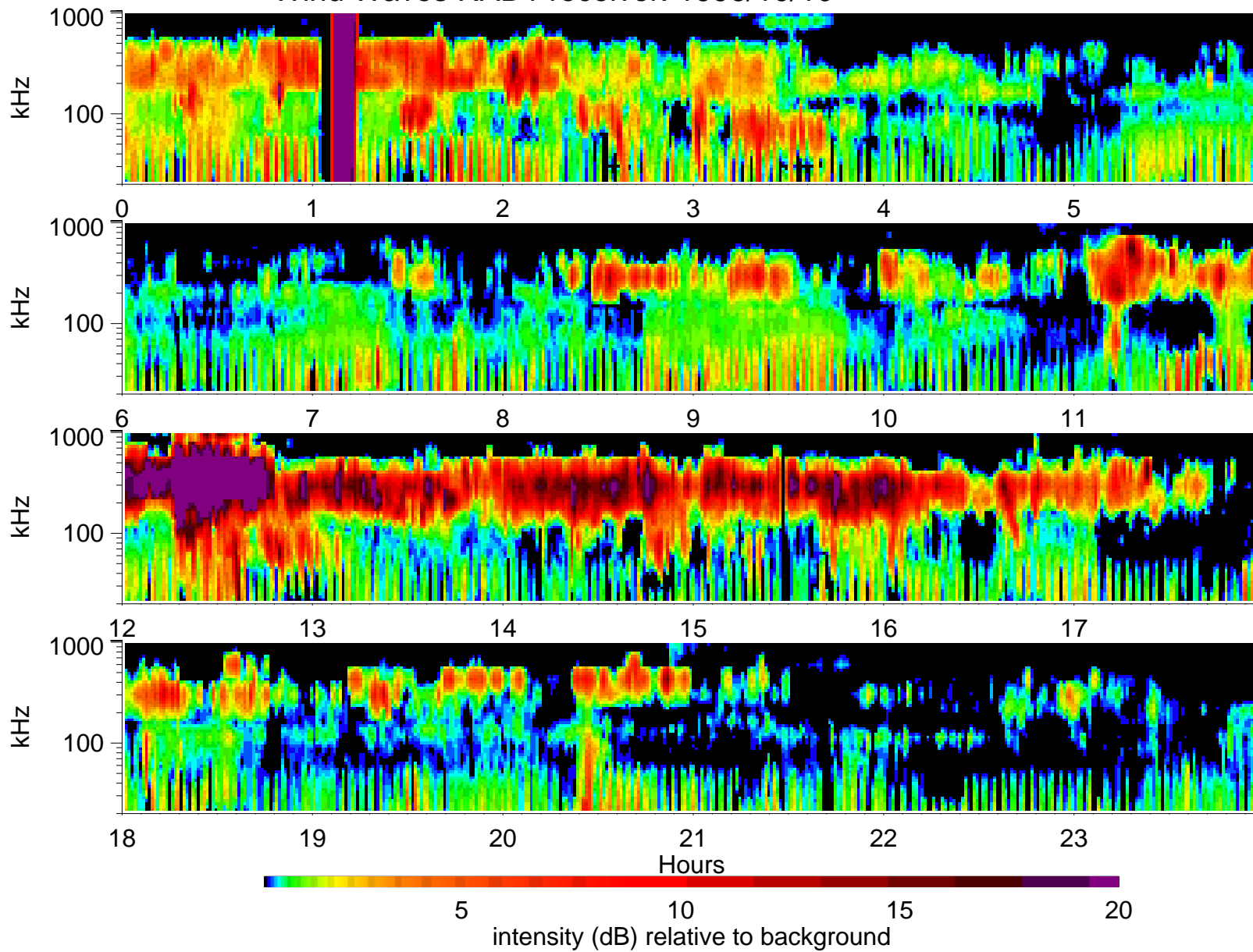
Wind Waves RAD1 receiver: 1996/10/10
