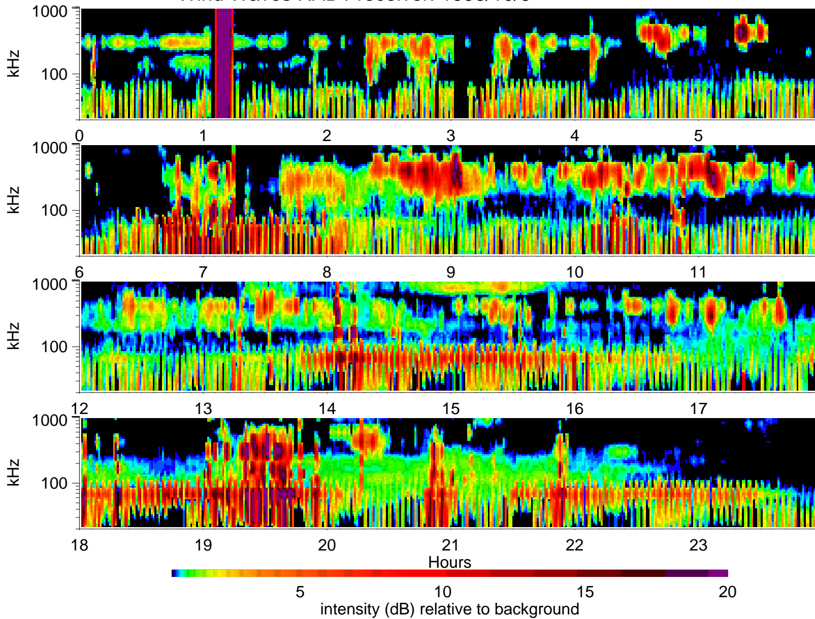
Wind Waves RAD1 receiver: 1996/10/6
