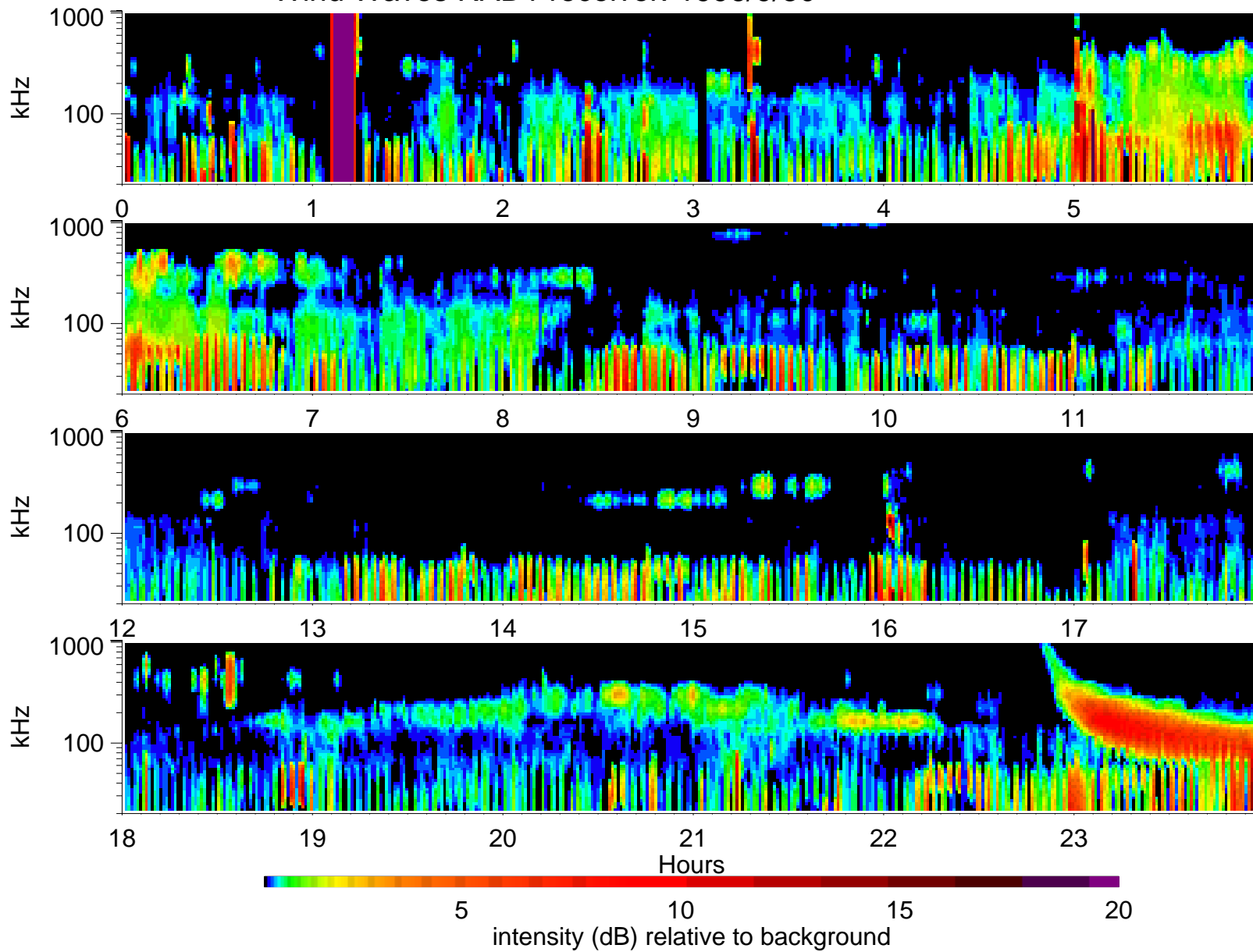
Wind Waves RAD1 receiver: 1996/9/30
