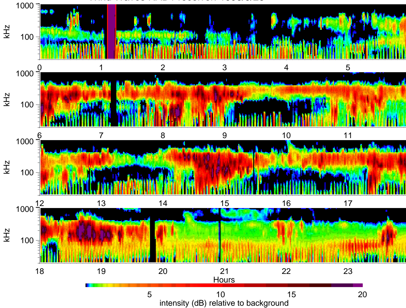
Wind Waves RAD1 receiver: 1996/9/28
