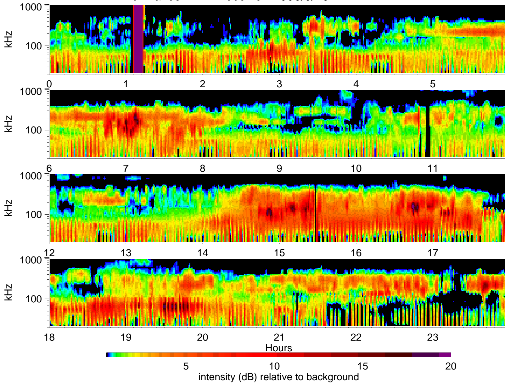
Wind Waves RAD1 receiver: 1996/9/26
