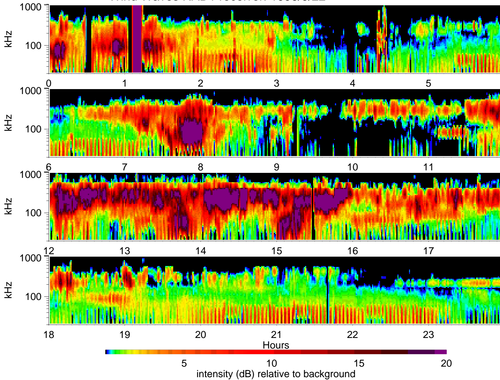
Wind Waves RAD1 receiver: 1996/9/22
