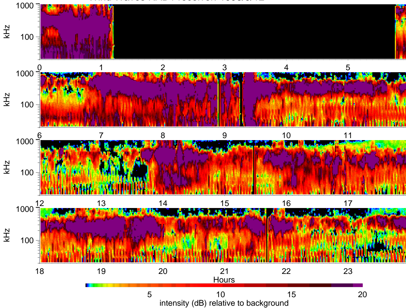
Wind Waves RAD1 receiver: 1996/9/12
