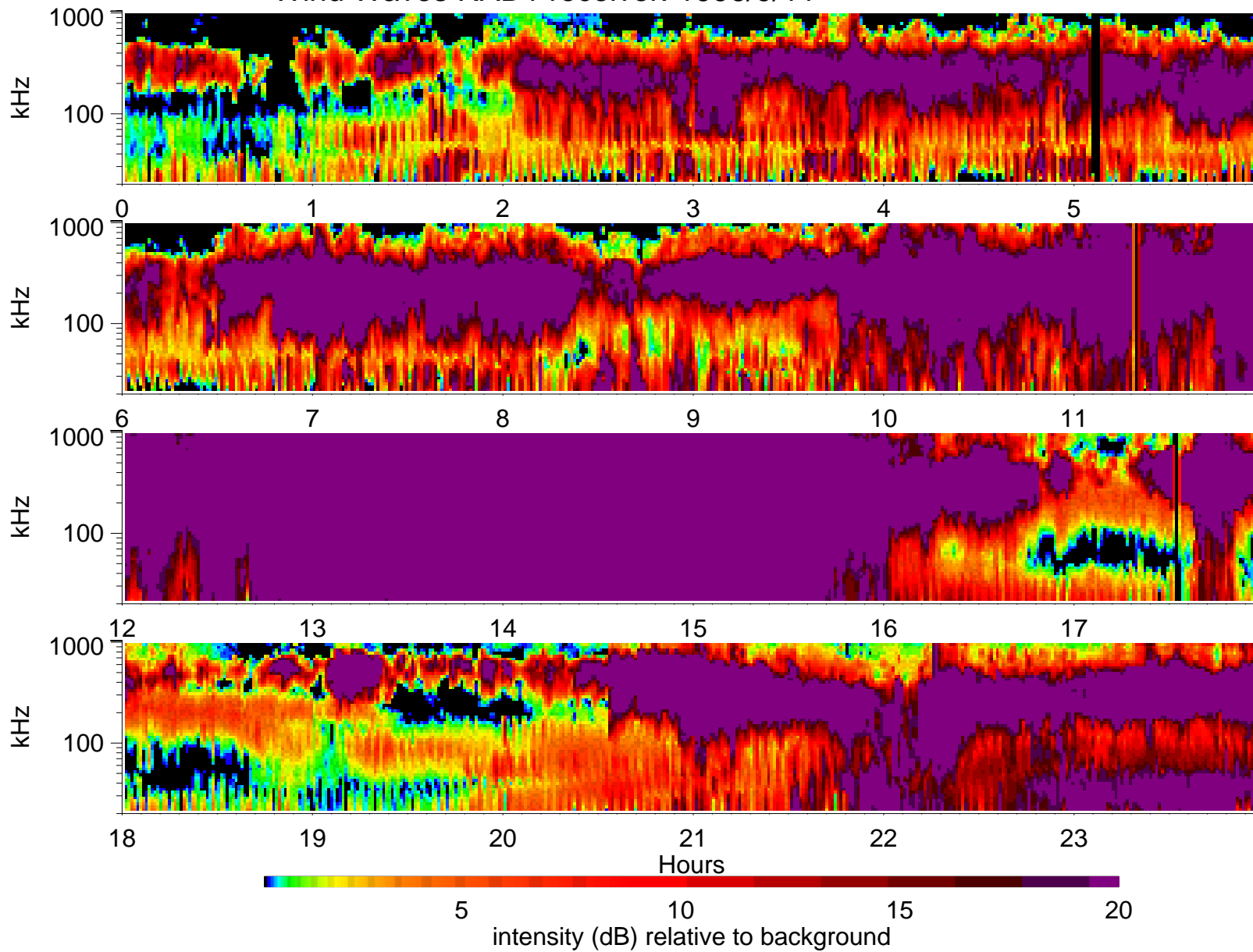
Wind Waves RAD1 receiver: 1996/9/11
