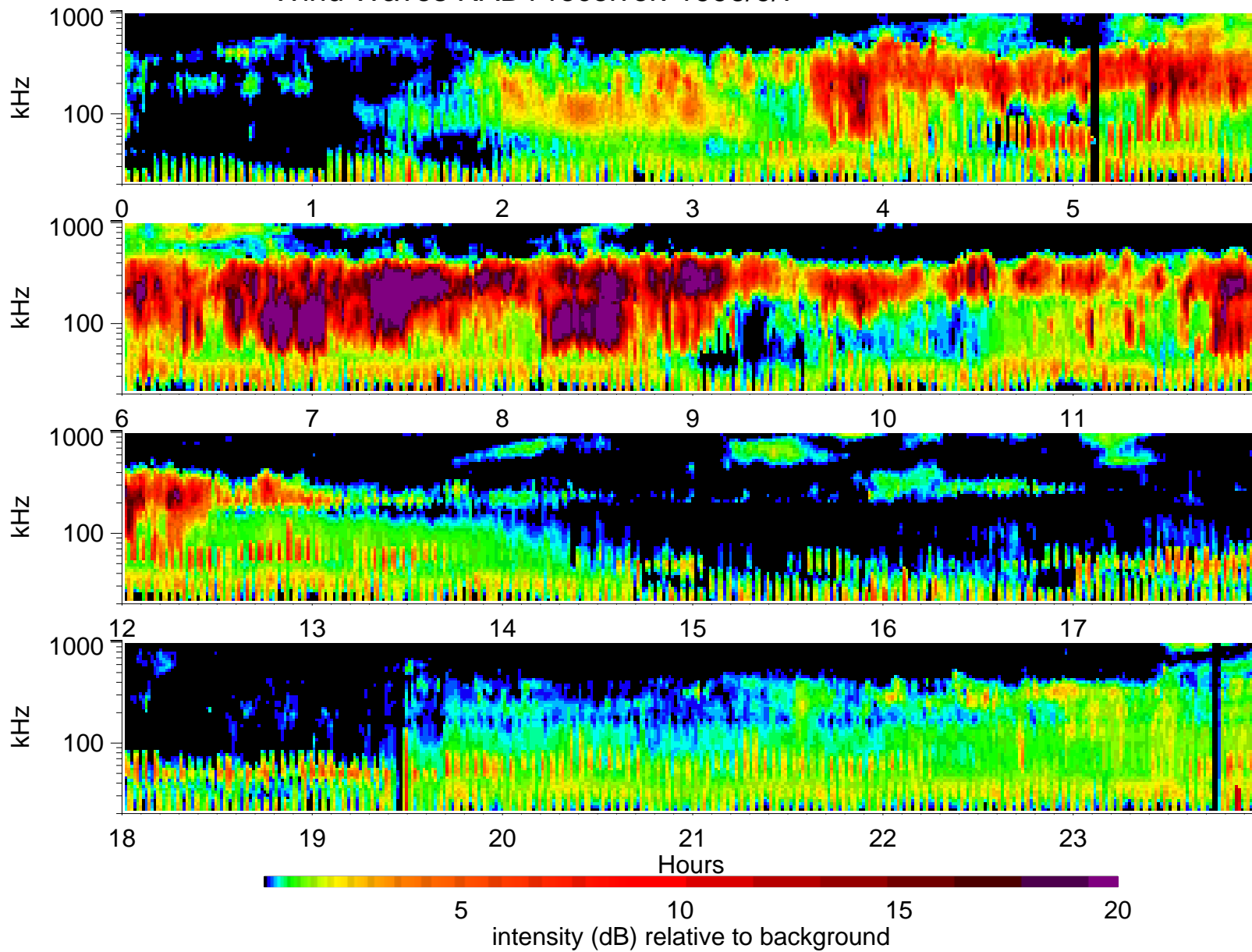
Wind Waves RAD1 receiver: 1996/9/7
