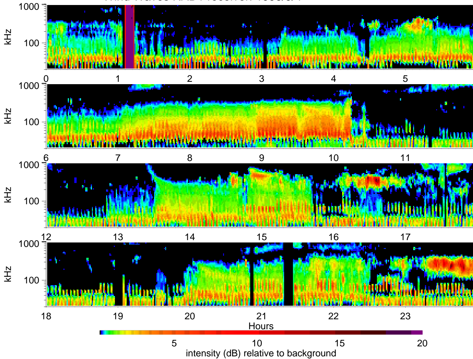
Wind Waves RAD1 receiver: 1996/9/4
