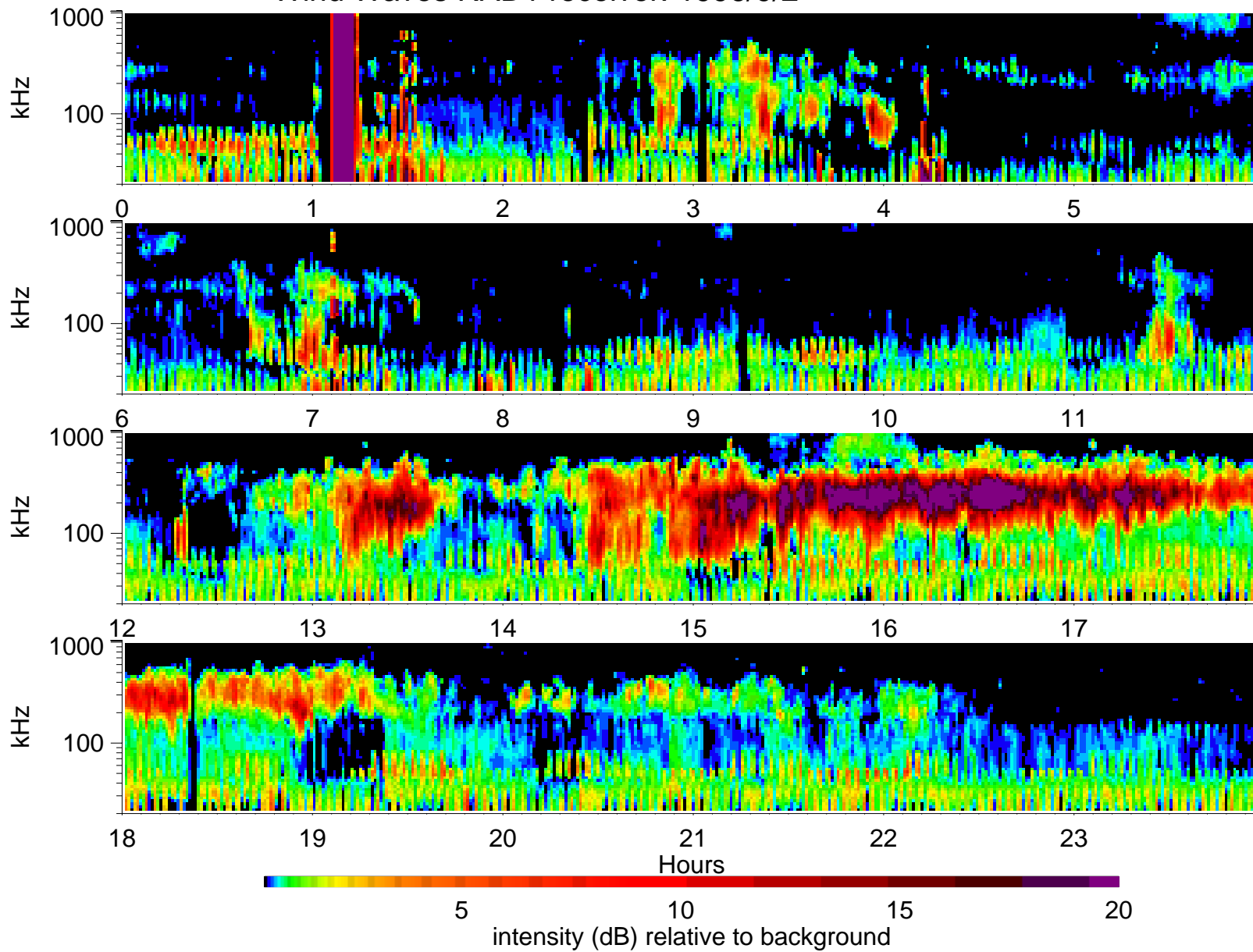
Wind Waves RAD1 receiver: 1996/9/2
