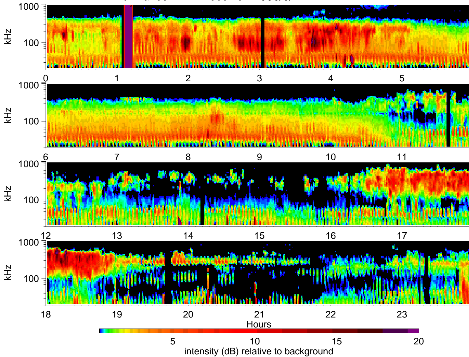
Wind Waves RAD1 receiver: 1996/8/27
