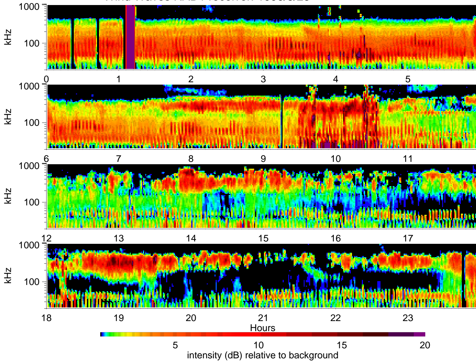
Wind Waves RAD1 receiver: 1996/8/23
