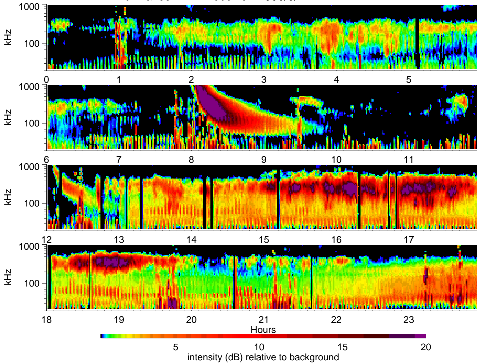
Wind Waves RAD1 receiver: 1996/8/22
