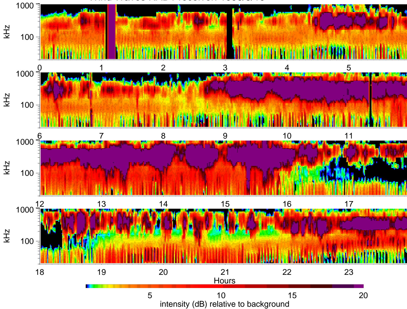
Wind Waves RAD1 receiver: 1996/8/19
