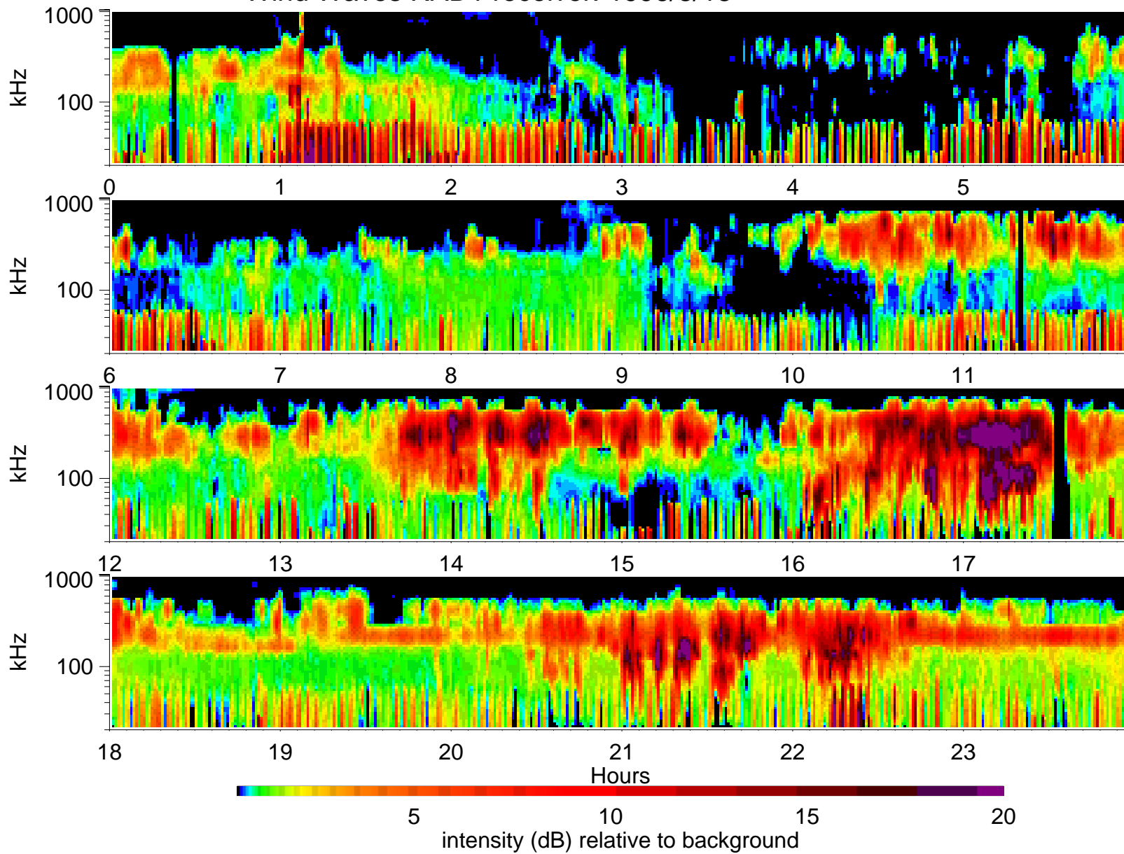
Wind Waves RAD1 receiver: 1996/8/18
