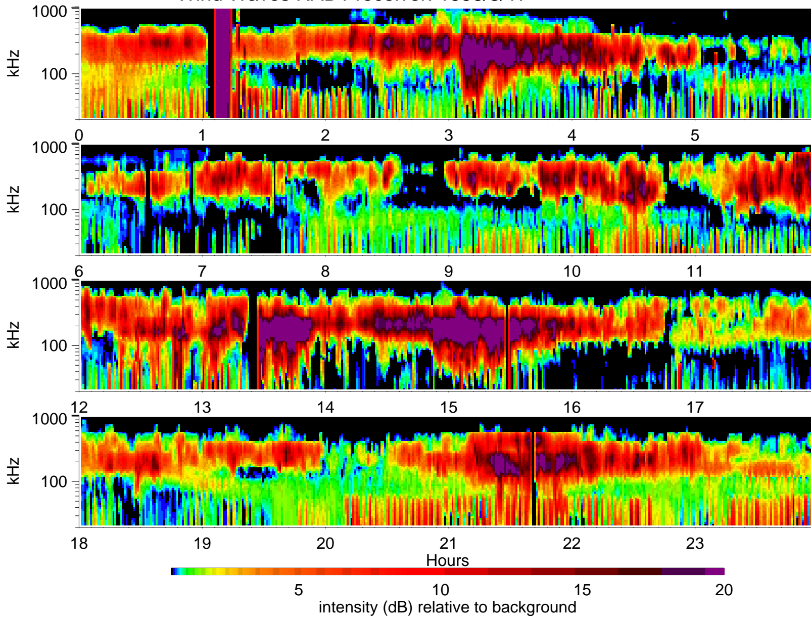
Wind Waves RAD1 receiver: 1996/8/17
