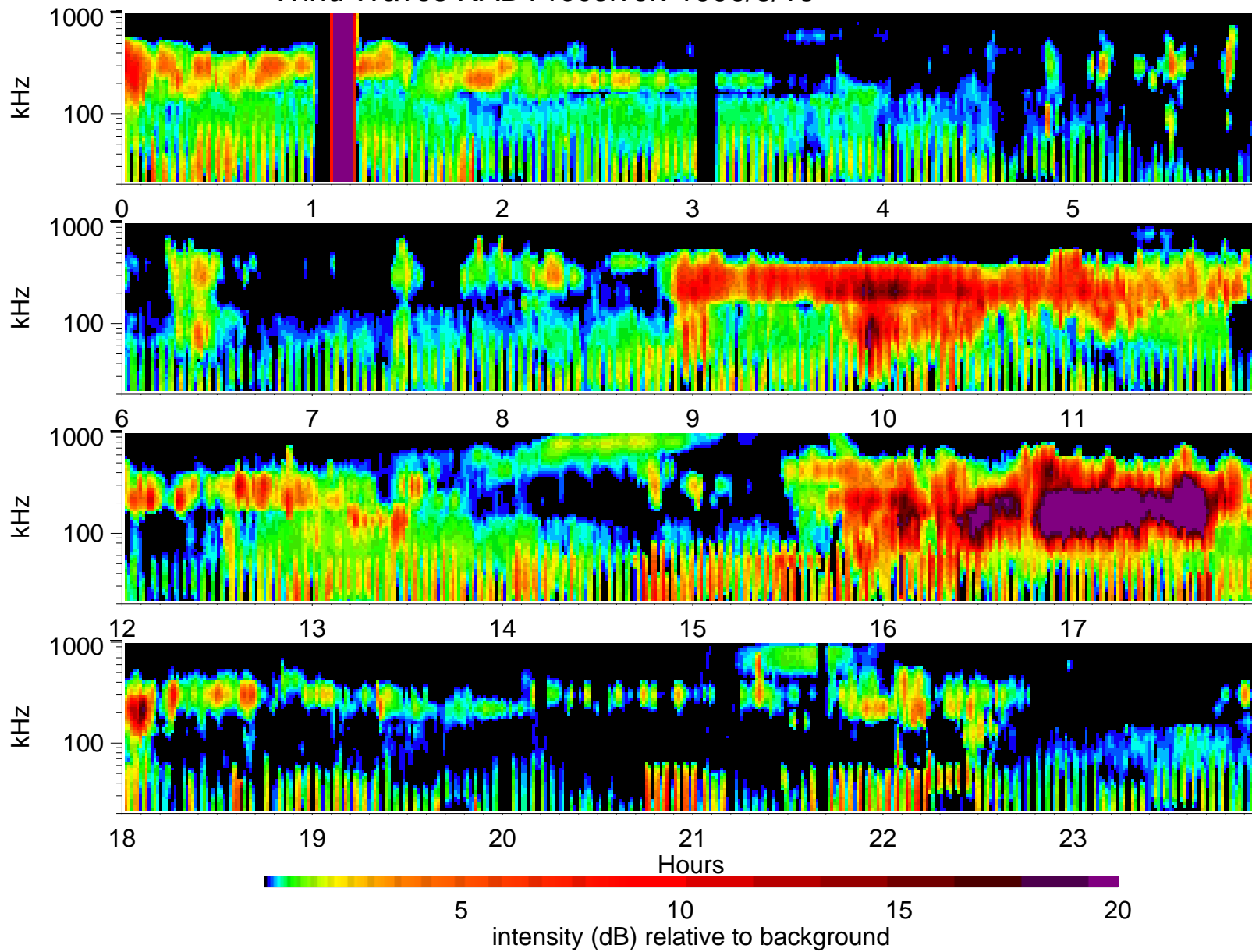
Wind Waves RAD1 receiver: 1996/8/15
