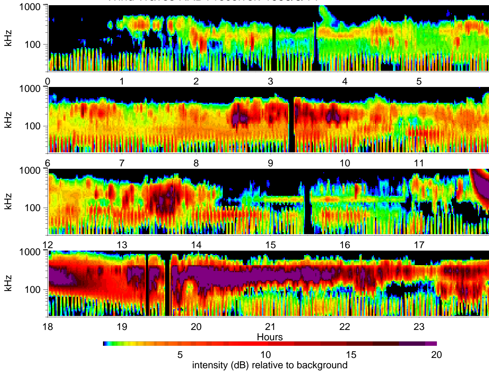
Wind Waves RAD1 receiver: 1996/8/14
