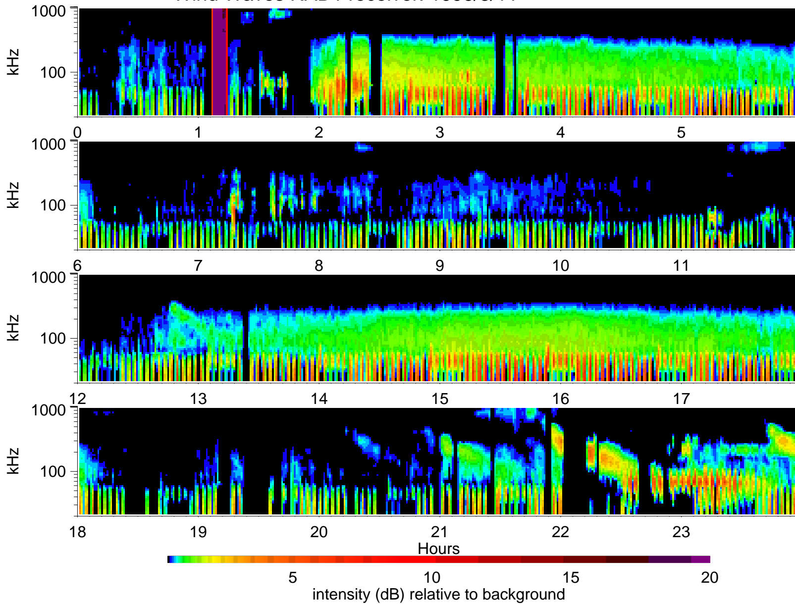
Wind Waves RAD1 receiver: 1996/8/11
