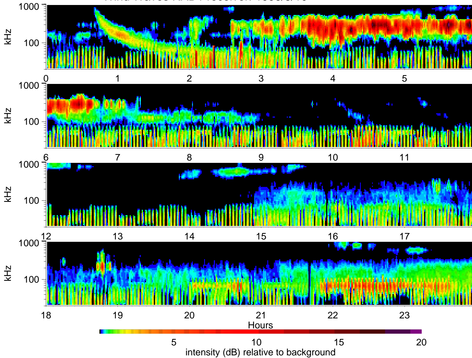
Wind Waves RAD1 receiver: 1996/8/10
