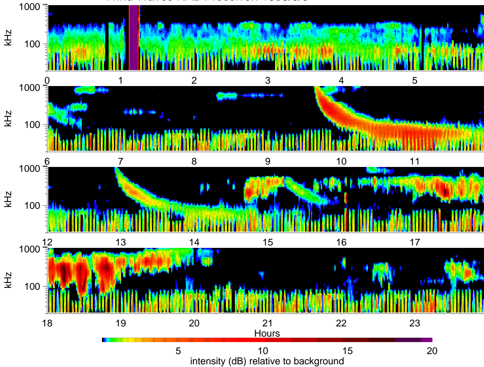
Wind Waves RAD1 receiver: 1996/8/9
