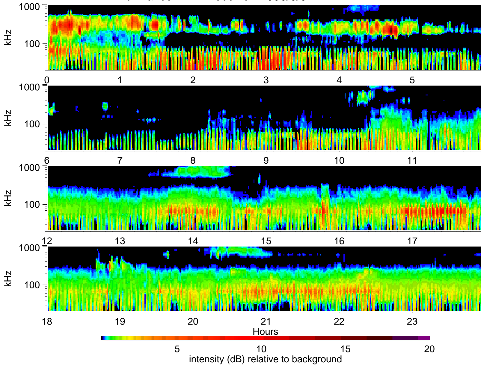
Wind Waves RAD1 receiver: 1996/8/8
