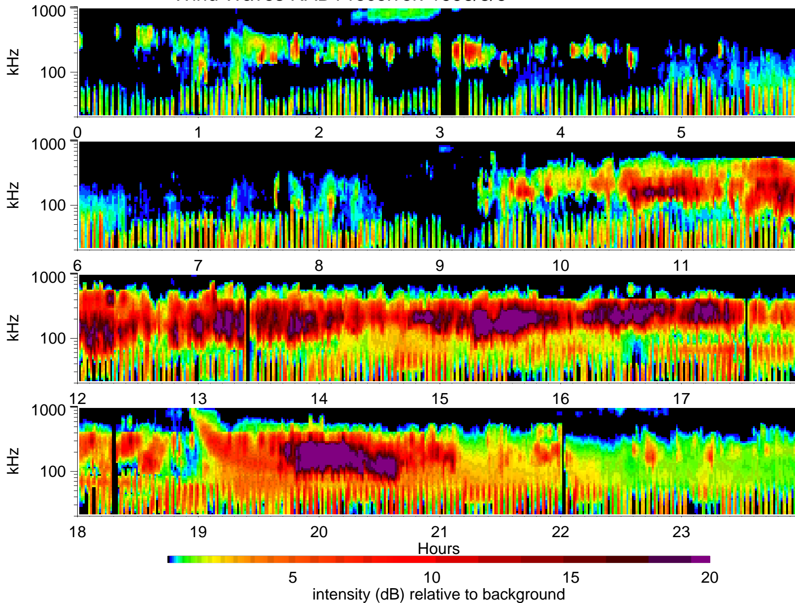
Wind Waves RAD1 receiver: 1996/8/6
