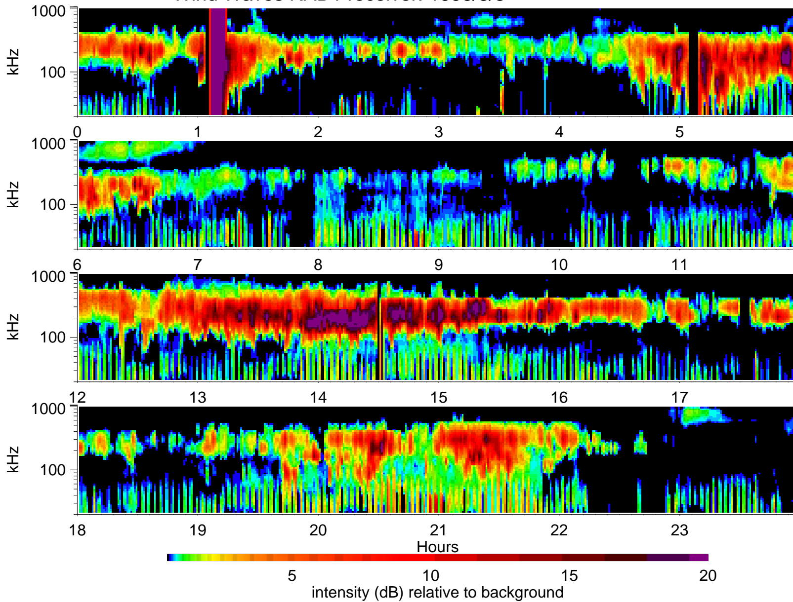
Wind Waves RAD1 receiver: 1996/8/5
