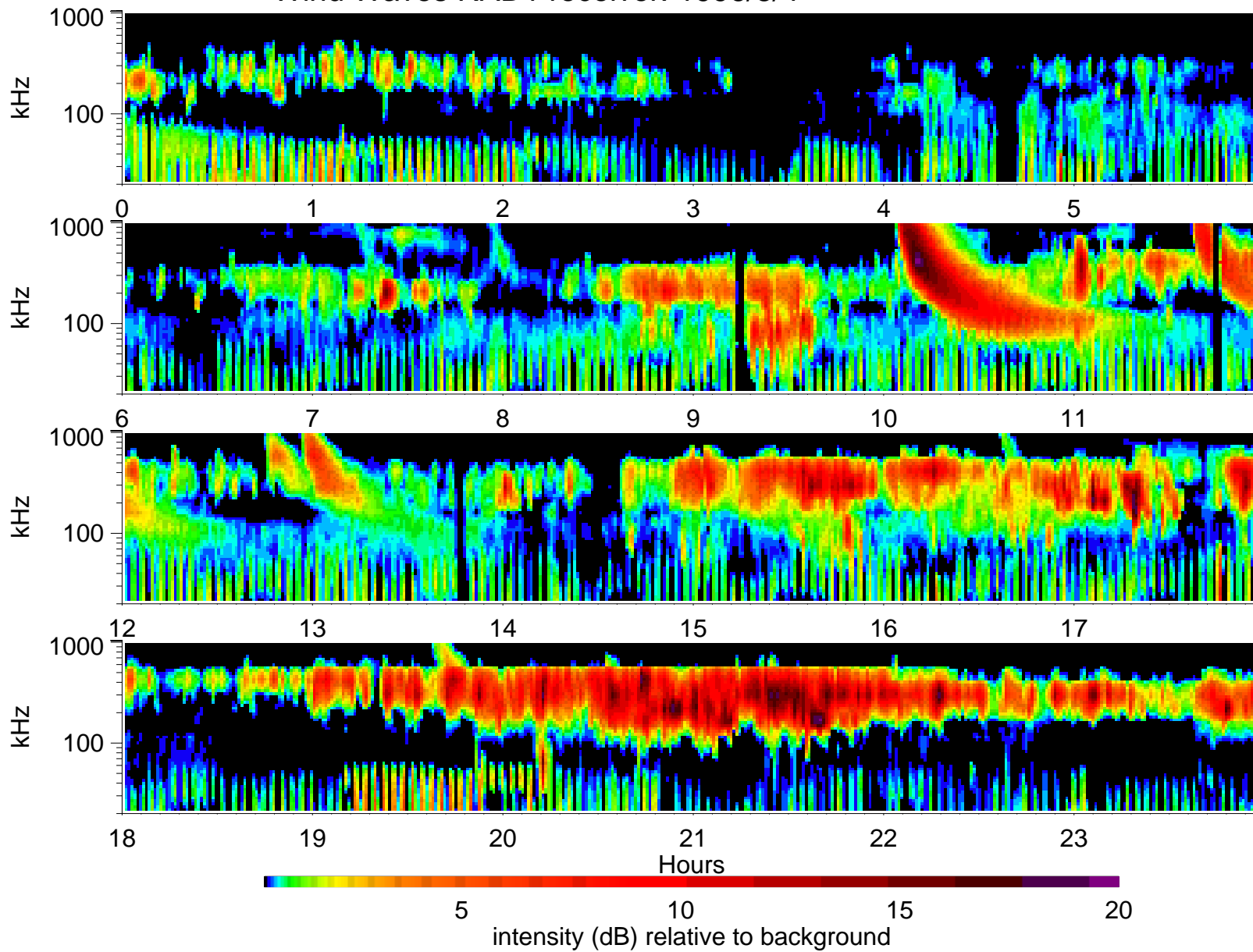
Wind Waves RAD1 receiver: 1996/8/4
