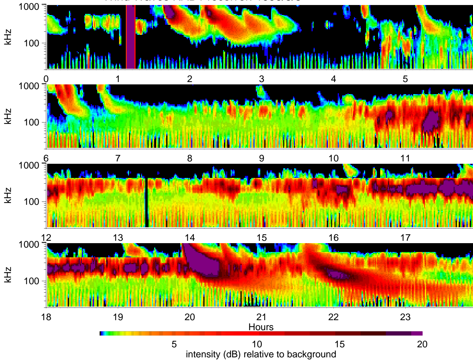
Wind Waves RAD1 receiver: 1996/8/3
