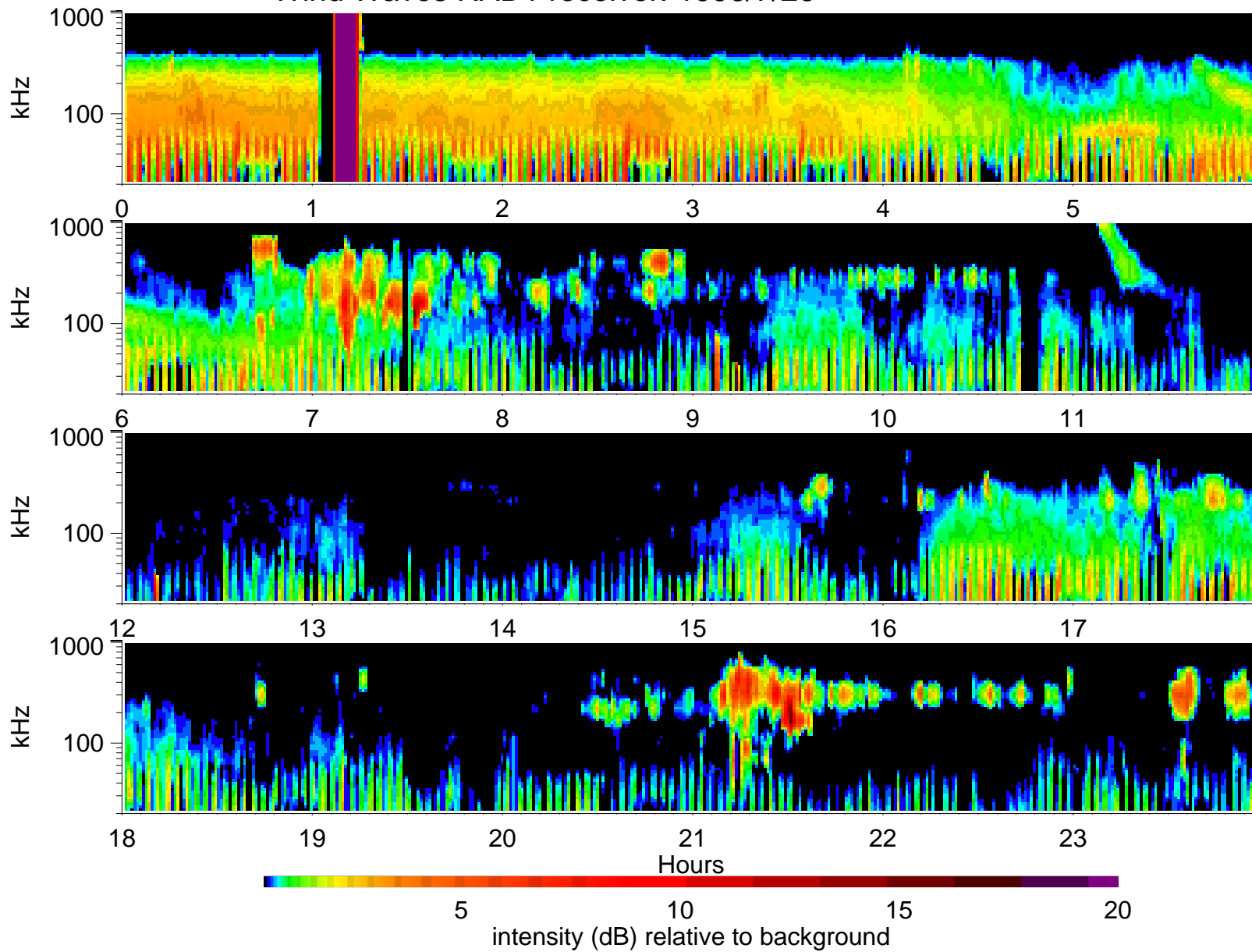
Wind Waves RAD1 receiver: 1996/7/26
