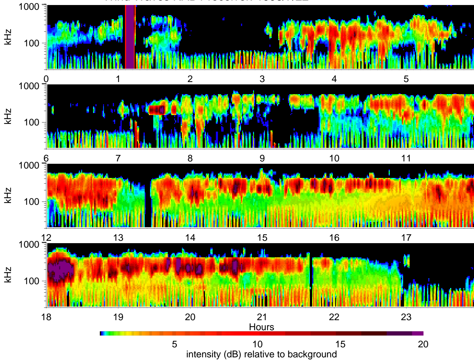
Wind Waves RAD1 receiver: 1996/7/22
