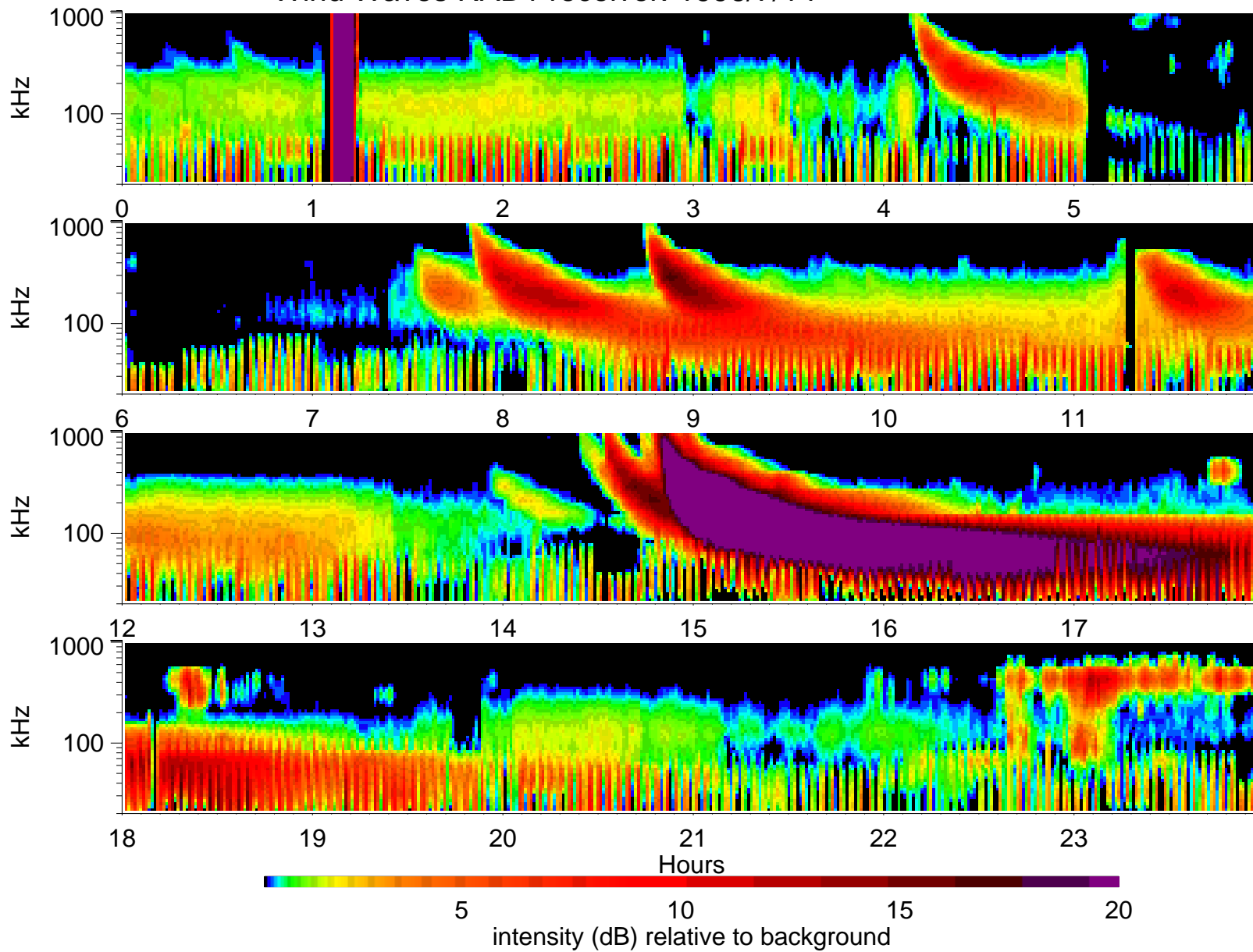
Wind Waves RAD1 receiver: 1996/7/14
